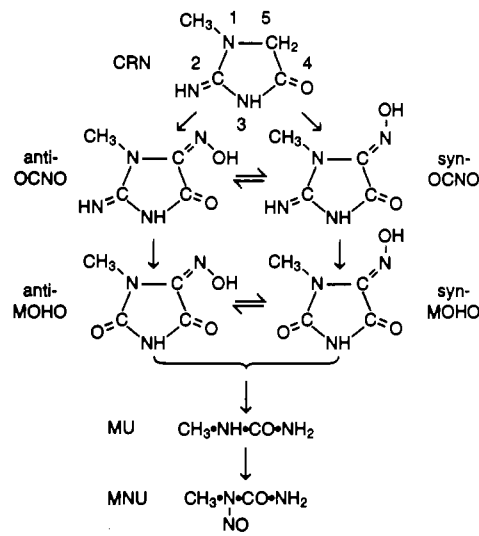
Scheme I. Structure (with Numbering) of CRN and Its Conversion by Nitrite to syn - and anti -OCNO and -MOHO and to MU and MNU
